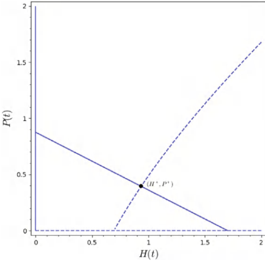
Figure 3.17: Numerical computation of the coexistence equilibrium point (H^*, P^*) .
