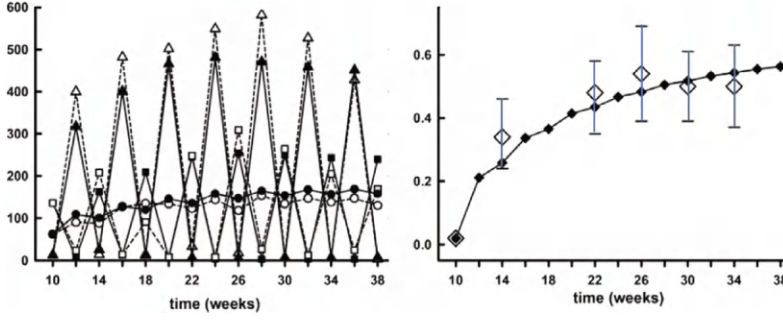
Figure 8.4: The black symbols in the left and right graphs show the time series of \mathbf{x}(t) = (x_1, x_2, x_3)^T and u(t) for the solution of the Darwinian LPA model with projection matrix (8.25) and trait-dependent components (8.26) with parameter values c_{pa} = 0.015 , c_{el} = 0.0093 , c_{ea} = 0.011 and \sigma^2 = 0.40 . The initial condition is \mathbf{x}(0) = (13, 136, 62)^T and u(0) = 0.02 . In the left graph, the triangles, squares, and circles are larvae x_1(t) , pupae x_2(t) , and adults x_3(t) , respectively. The open symbols in the left graph are data from one replicate of the experiment reported in [255] and the open diamonds in the right graph are the averaged +allele frequencies over all replicates (with error bars).
