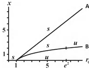
Figure 1.13: The bifurcation diagrams for A. the discrete logistic (Beverton–Holt) equation (1.25) (drawn with c = 1 ) and B. the exponential equation (1.29) (drawn with c = 1 ) in which the local stability properties of equilibria are indicated by s (locally asymptotically stable) and u (unstable).
