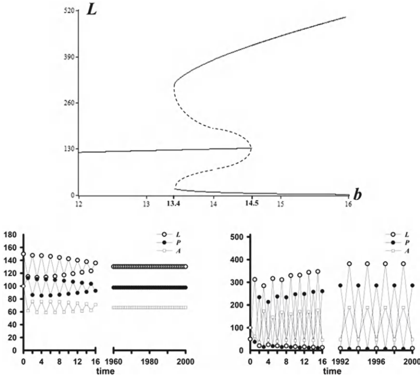
Figure 6.9: Shown is the bifurcation diagram for the LPA model with projection matrix (6.53), using b as the bifurcation parameter, and plotting the L component of the attractor. Parameter values are c_{el} = c_{eq} = c_{pa} = 0.01 , \mu_l = 0.25 , and \mu_a = 0.75 . The forward, stable bifurcation of positive equilibria occurs at b_0 = 1 (not shown) and a backward-unstable 2-cycle bifurcation occurs at b \approx 14.5 (the dotted lines). A saddle-node bifurcation occurs at b \approx 13.4 , giving rise to stable 2-cycles. For b in the interval 13.4 < b < 14.5 , there exist a stable positive equilibrium and a stable 2-cycle. This is illustrated by the two time series plots at b = 14 , one of which (with initial condition \mathbf{x}(0) = (150, 100, 100)^T ) tends to the equilibrium and the other of which (with initial condition \mathbf{x}(0) = (50, 100, 100)^T ) tends to a 2-cycle.
