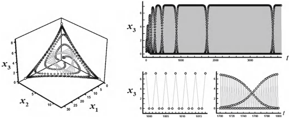
Figure 6.5: These graphs show a sample orbit and time series for the k = 3 dimensional semelparous Leslie model (6.49) with density factors \beta(w) = \sigma_i(w) = 1/(1+w) , competition coefficient matrix C = \begin{pmatrix} 0.01 & 0 & 0 \\ 0.03 & 0.01 & 0 \\ 0.01 & 0.02 & 0.01 \end{pmatrix} , and parameters b = 4 , s_1 = 0.5 , s_2 = 0.75 , which imply R_0 = 1.5 and (\rho_1, \rho_2) = (2.133, 0.5333) \in \Omega_3 . In the three-dimensional plot on the left, the orbit with initial condition \mathbf{x}(0) = (1, 1, 1) in the interior \mathring{\mathbb{R}}_+^3 (the open square) is seen tending, in an outward spiraling fashion, to a heteroclinic cycle of type A lying on the boundary \partial R_+^3 . The top plot on the right shows the time series for the adult component x_3 of the orbit. The lower two graphs show, left to right, respectively, an episode of synchronous 3-cycle dynamics and an episode showing a transitional shift from one phase to another phase of the 3-cycle. Figures reproduced with permission from [71].
