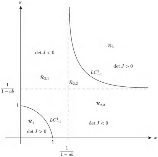
Figure 3.27: The set of singular points of the Ricker competition model consists of two branches, the lower curve LC^1_{-1} and the upper curve LC^2_{-1} .
