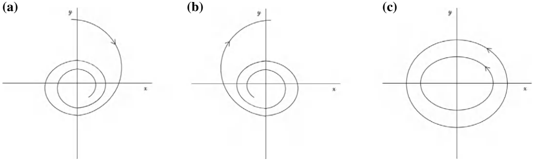
Figure 3.3: (a) stable focus: |\lambda| < 1 . (b) source: |\lambda| > 1 . (c) center: |\lambda| = 1 .
