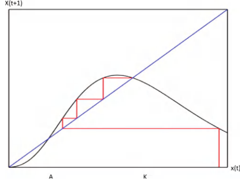
Figure 1.14: The cobweb diagram of the Ricker model with the strong Allee effect. There are three equilibrium point x_1^* = 0 , which is asymptotically stable, the Allee equilibrium point A , which is unstable, and the carrying capacity K , which is asymptotically stable.
