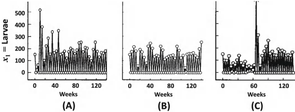
Figure 9.2: Shown are plots of the larval component of some sample replicates taken from data gathered in replicated and controlled experiments with flour beetles that were designed to corroborate the model predictions of the periodically forced LPA model. In (A) the habitat is held constant and the model predicts a stable 2-periodic solution (alternating between 0 and a high of 162). When the habitat oscillates with amplitude \alpha = 0.4 the model predicts a resonant 2-periodic solution in-phase with the habitat and an attenuant 2-periodic solution out-of-phase with the habitat. The initial conditions in (B) and (C) predict approach to the former and latter 2-periodic solutions, respectively. Notice that the replicated in (C) switches from the attenuant to the resonant solution due to a stochastic event that moves it to the resonant solution's basin of attraction.
