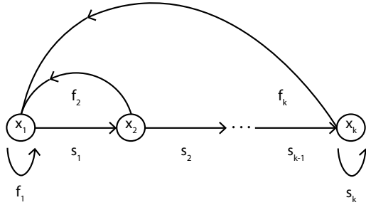
Figure 2.2: The life cycle graph for a general Leslie matrix.
