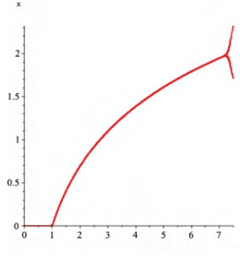
Figure 1.16: The bifurcation diagram of the exponential map, at b = 1 we have a transcritical bifurcation, and at b = e^2 , we have period-doubling bifurcation.
