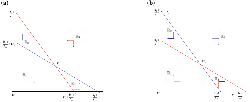
Figure 3.11: (a) In the first scenario, \frac{c_{12}}{c_{22}} < \frac{b_1-1}{b_2-1} < \frac{c_{11}}{c_{21}} , the orbits stay in the neighborhood of the equilibrium point E_4^* . (b) In the second scenario, \frac{c_{11}}{c_{21}} < \frac{b_1-1}{b_2-1} < \frac{c_{12}}{c_{22}} , the orbits do not stay in the neighborhood of the equilibrium point E_4^* , and thus E_4^* is unstable.
