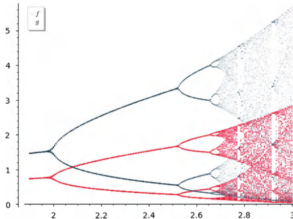
Figure 3.34: The figure illustrates the phenomenon of period-doubling route to chaos. The Ricker map F is written as F = (f, g)^T . The figure shows a bifurcation diagram, on the x -axis we have the parameter \alpha and on the y -axis we have the omega limit sets of both the x -components and the y -components of the orbits.
