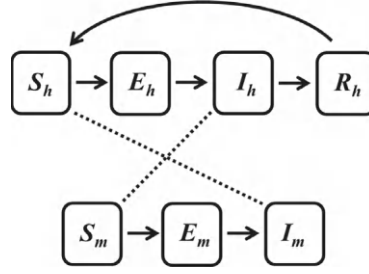
Figure 7.7: The dashed lines shown represent the interactions between infectious and susceptible individuals. Not shown are the in-flows into the susceptible classes due to births.
