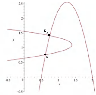
(c) a_1 = 2.5 , a_2 = 2.2 , b_1 = 0.22 , b_2 = 0.15 Two interior equilibria.
