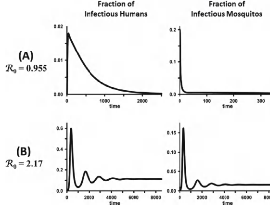
Figure 7.8: Plotted are I_h(t)/N_h(t) and I_m(t)/N_m(t) for a sample solution of the malaria model (7.76) with the unit of time equal to one day. Parameters (adapted from those in [50]) are: \nu_{Rh} = 0.005 , \nu_{Eh} = 0.1 , \nu_{Ih} = 0.0015 , \nu_{Em} = 0.1 , \sigma_{Sh} = 0.999 , \sigma_{Rh} = 0.999 , \sigma_{Eh} = 0.999 , \sigma_{Ih} = 0.98 , \sigma_{Sm} = 0.95 , \sigma_{Em} = 0.95 , \sigma_{Im} = 0.95 , b_h = 0.005 , b_m = 10 , c_h = 0.0001 , c_m = 0.001 , \beta_{hm} = 0.2 , \beta_{mh} = 0.4 , \sigma_m = 0.5 . (A) \sigma_h = 0.36 with all initial conditions equal to 0 except S_h(0) = 40,000 , S_m(0) = 9,900 , and I_m(0) = 100 . (B) \sigma_h = 1 with all initial conditions equal to 0 except S_h(0) = 40,000 , S_m(0) = 8,000 , and I_m(0) = 2,000 .
