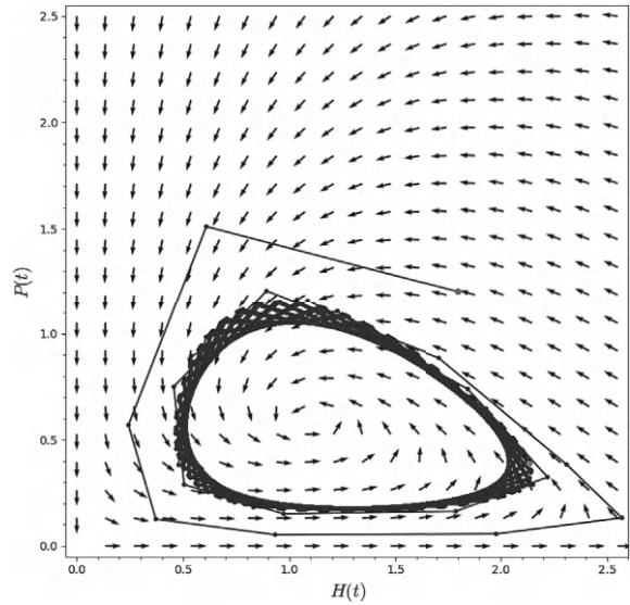
Figure 3.37: Phase space diagram for the parameters r = 1.25 , \alpha = 1 , c = 1 , and K = 2.7 .
