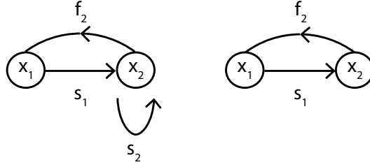
Figure 2.7: The life cycle graphs for the Leslie matrix models in Example 29.
