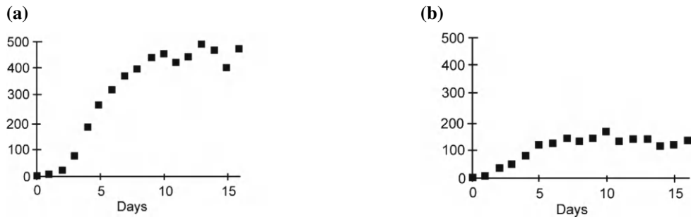
Figure 3.9: (a) Time series for the growth of P. Aurelia alone. (b) Time series for the growth of P. Caudatum alone.
