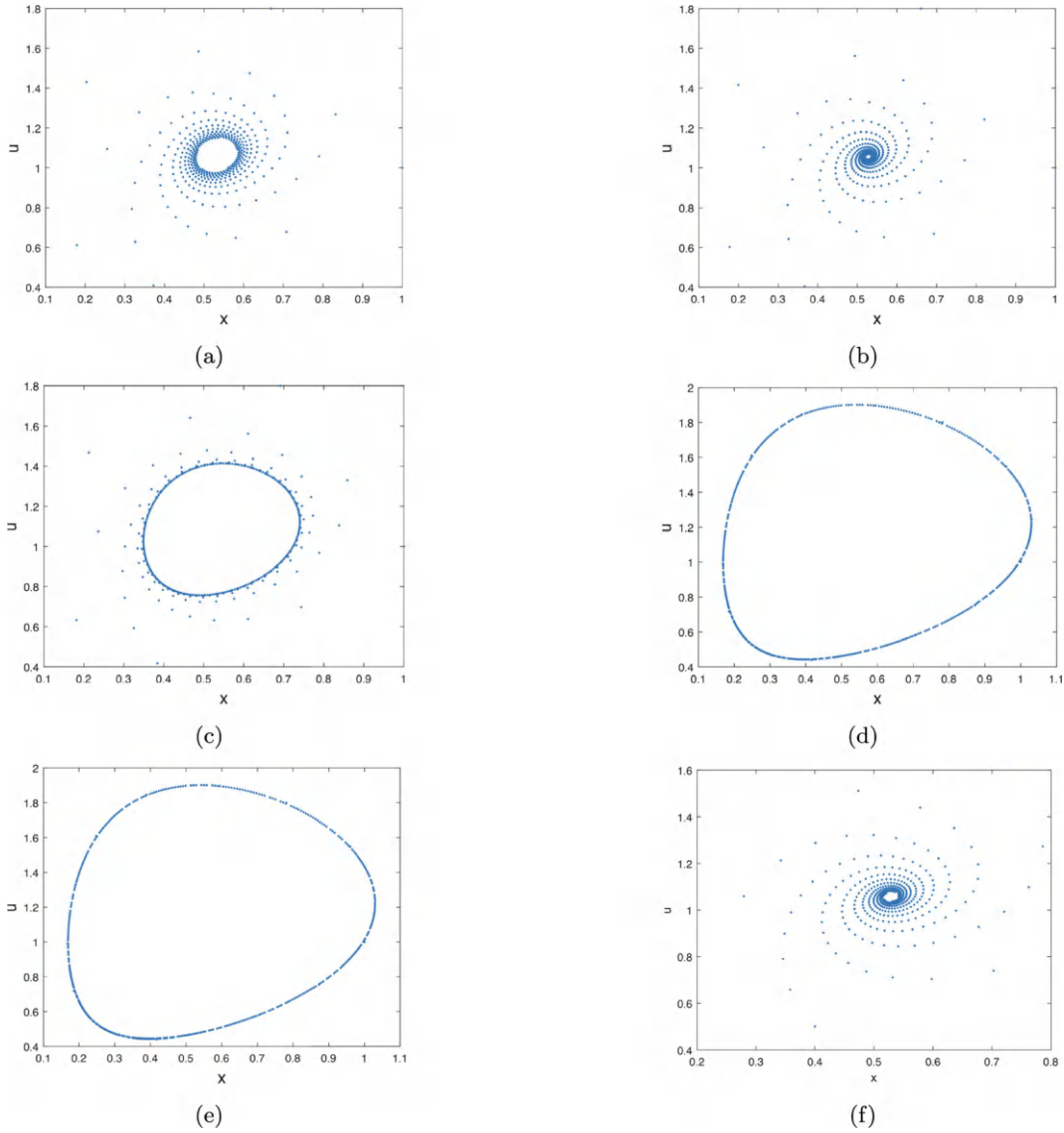
Figure 8.12: Supercritical Neimark-Sacker bifurcation diagram of the evolutionary Ricker model, under the assumption that c_0 = 1 .
