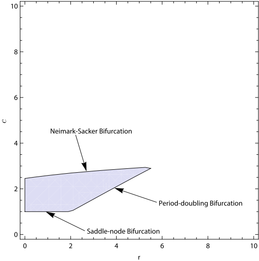
Figure 3.18: The figure depicts the parameter space r - c bifurcation diagram. The equilibrium E_3^* = (H^*, P^*)^T is asymptotically stable when the parameters r and c are in the shaded region.
