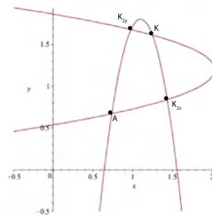
(g) a_1 = 2.2 , a_2 = 2.46 , b_1 = 0.11628 , b_2 = 0.21628 Four interior equilibria.
