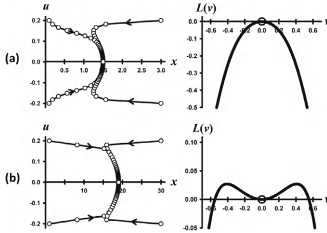
Figure 8.1: Phase plane orbits and adaptive landscapes are shown for two examples of (8.9) and (8.10) with parameter values w_0 = 5 , w_1 = 5.5 , c_0 = 1 , s_a = 0.25 , s_n = 0.5 , and \sigma^2 = 0.01 . (a) b = 5 : four typical orbits in the x, u -phase plane approach the equilibrium (x^*, u^*)^T = (1.5, 0)^T . The adaptive landscape L(v) has a global maximum at v = 0 and the trait component of the positive equilibrium is an ESS. In this case, inequality (8.17) fails. (b) b = 40 : four typical orbits in the x, u -phase plane approach the positive equilibrium (x^*, u^*)^T = (19.0, 0)^T . The adaptive landscape L(v) has a local minimum at v = 0 and the trait component of the positive equilibrium is not an ESS. In this case inequality (8.17) holds. Figure reproduced from [81] with permission.
