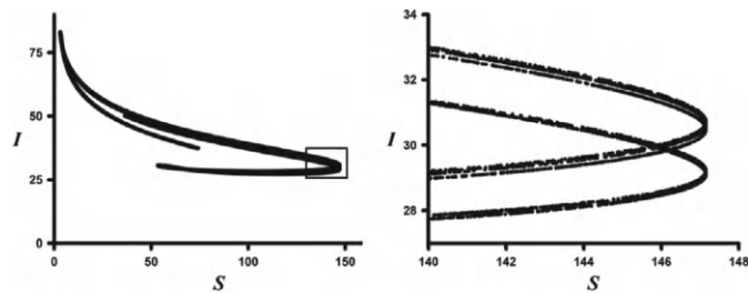
Figure 7.3: A strange attractor from the bifurcation diagram in Figure 7.2 with \mathcal{R}_0 = 18 . Shown are 50,000 points from the orbit with initial condition (S(0), I(0))^T = (50, 40) after the first 1,000 initial transient points are excluded. Also shown is a blow-up view of the indicated piece of the attractor.
