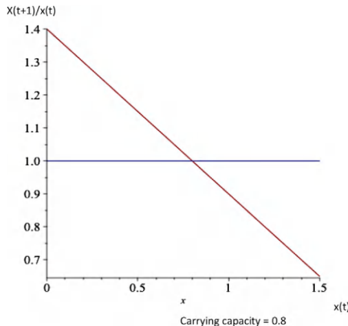
Figure 1.5: The population growth rate function of the quadratic model.
