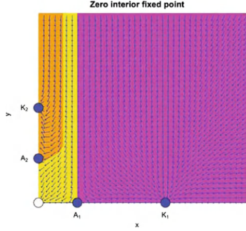
Figure 5.17: The phase space diagram in the case of no interior fixed points. The domain \mathbb{R}_+^N is divided into three regions, an extinction region (yellow), an exclusion region of y (magenta), and an exclusion regions of x (orange). Note that the extinction region is unbounded.
