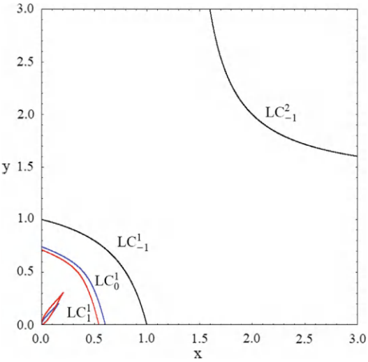
Figure 3.28: The images LC^1_0 and the upper curve LC^2_0 of LC^1_{-1} and the upper curve LC^2_{-1} , respectively, are shown.
