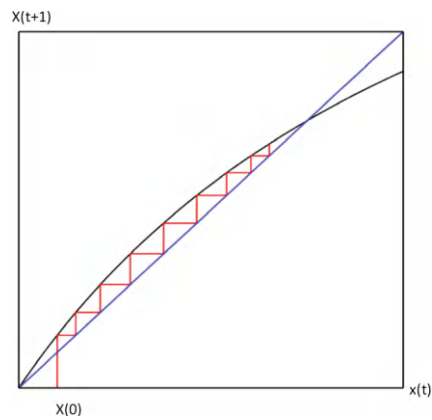
Figure 1.9: The cobweb diagram of the discrete logistic map, where b > 1 . The population size approaches the equilibrium point.
