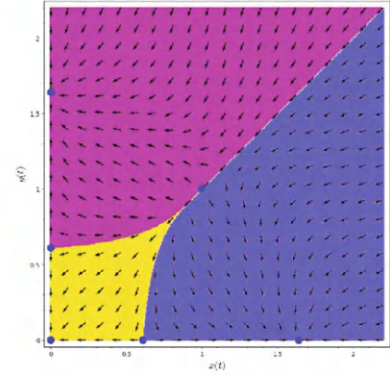
(b) one interior equilibrium point
