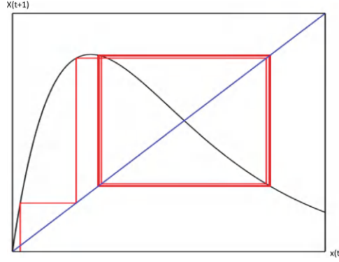
Figure 1.18: The appearance of a 2-cycle in the exponential map when b > e^2 .
