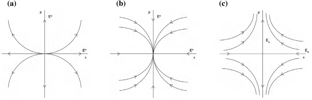
Figure 3.1: (a) unstable node: \lambda_1 > \lambda_2 > 1 . (b) stable node: -1 < \lambda_1 < \lambda_2 < 1 . (c) saddle: -1 < \lambda_1 < 1, \lambda_2 < 1 .
