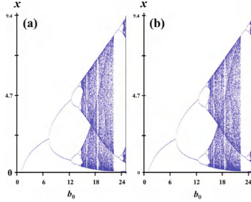
Figure 8.6: (a) The familiar bifurcation diagram for the Ricker equation x(t+1) = b_0 \exp(-c_0 x_t) x_t with c_0 = 1 (b) The bifurcation diagram showing the x component of the Darwinian Ricker equation (8.30) with c_0 = 1 and \sigma^2 = 1 .
