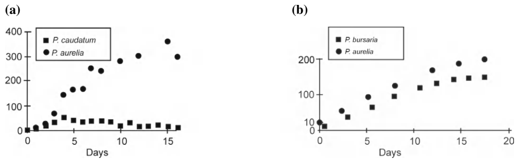
Figure 3.10: (a) P. Aurelia out competes P. Caudatum . (b) P. Aurelia coexists with P. Bursaria .
