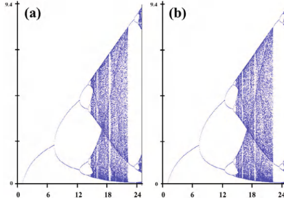
Figure 8.10: (a) The familiar bifurcation diagram for the Ricker equation (3.55)a with c_0 = 1 , (b) The bifurcation diagram showing the x component of the Darwinian Ricker equation with c_0 = 1 , c_1 = 0 and \sigma^2 = 1 .
