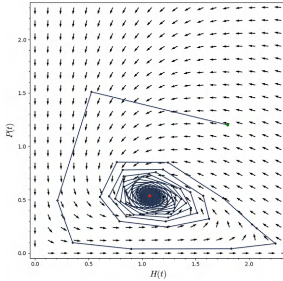
Figure 3.35: Phase space diagram for the parameters r = 1.25 , \alpha = 1 , c = 1 , and K = 2.5 .
