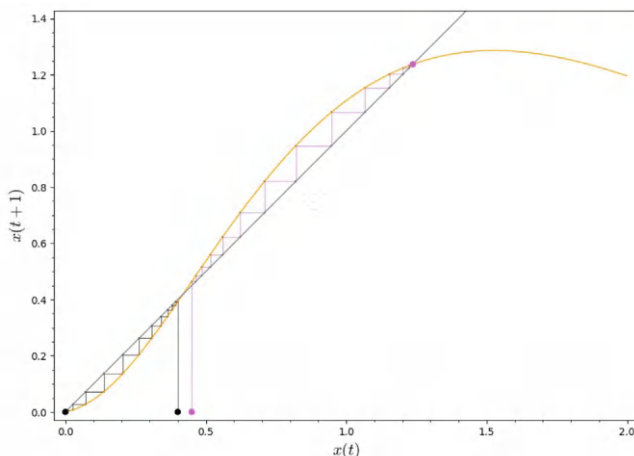
Figure 5.6: If the population density goes below the Allee threshold A , the the population will go extinct. The population may persist if its initial density is above the Allee threshold.
