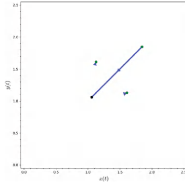
Figure 5.3: The graph shows one locally asymptotically 2-cycle and two asymptotically stable equilibrium points.
