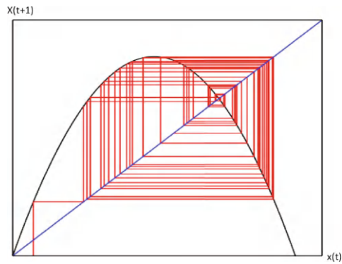
Figure 1.20: An unstable 2-cycle, r > \sqrt{6} .
