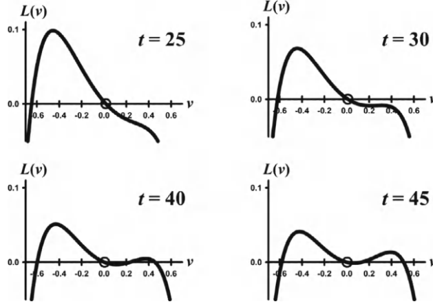
Figure 8.2: Selected time snapshots of the adaptive landscape are shown for the orbit (x(t), u(t))^T with initial condition (x(0), u(0))^T = (30, 0.2)^T in the simulation shown in Figure 8.1(b). The trait component u(t) moves to the left, uphill toward the peak on the left (not easily perceptible on the scale shown), but nonetheless asymptotically arrives at a local minimum on the equilibrium landscape (shown in Figure 8.1(b)). Figure reproduced from [81] with permission.
