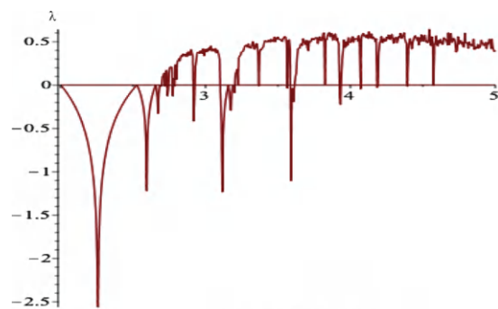
Figure (a): Liapunov Exponent
