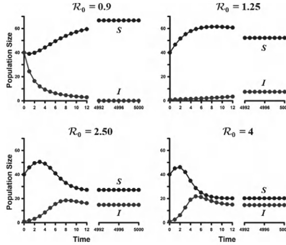
Figure 7.1: Sample solution time series obtained from (7.22) with b = 3/2 , c = 3/100 , \sigma_S = 1/2 and \sigma_I = 2/5 . Upper left: c_\varphi = 1.08 . Upper right: c_\varphi = 1.5 . Lower left: c_\varphi = 3 . Lower right: c_\varphi = 4.8 .
