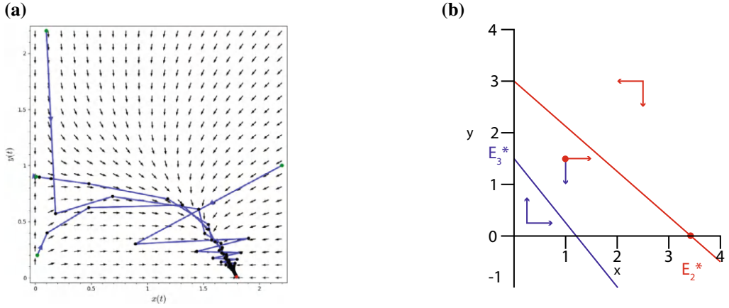
Figure 3.15: (a) The equilibrium points E_2^* is locally asymptotically stable and E_3^* is a saddle. (b) The isoclines do not intersect in the interior of R_+^2 . The orientation of the orbits indicate that E_2^* is most likely asymptotically stable.
