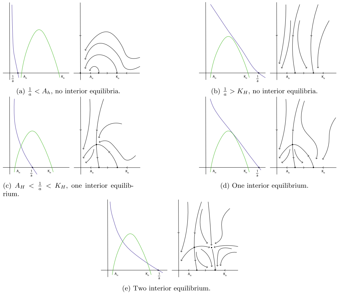
Figure 5.15: The five possible scenarios of the existence and stability of the interior equilibria. The interior equilibria are the intersection points of the two isoclines. Associated are the phase space diagrams depicting the global dynamics of the system.
