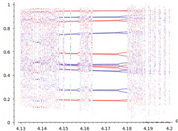
Figure 3.43: At a \approx 4.165 a 5-cycle appears and at a \approx 4.2 , both species go the extinction.
