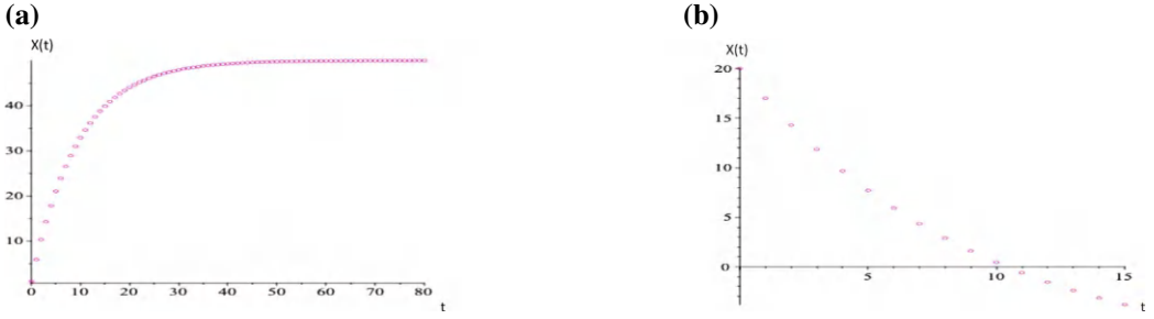
Figure 1.2: (a) The population with migration (stocking) grows to its carrying capacity (equilibrium), when r < 1 and m > 0 . (b) The population with immigration goes to extinction when r < 1 and m < 0 .
