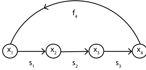
Figure 2.5: The life cycle graph of the Leslie matrix model in Example 23.
