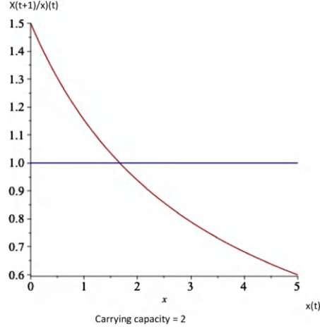
Figure 1.3: The population growth rate function of the discrete logistic (Beverton–Holt) model.
