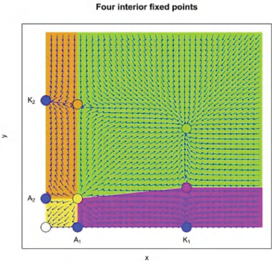
Figure 5.19: The phase space diagram in the case of four interior fixed points. The domain \mathbb{R}_+^N is divided into four regions, an extinction region (yellow), an exclusion region of y (magenta), an exclusion region of x (orange), and a coexistence region (green).
