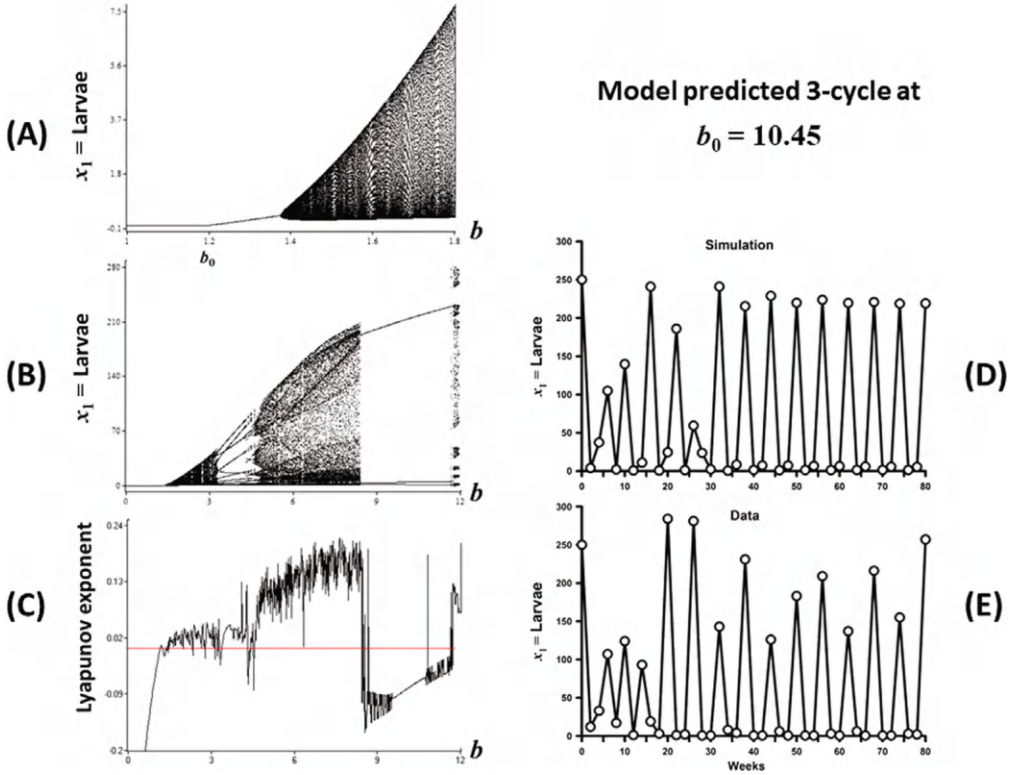
Figure 6.10: Conditioned least square estimates for the LPA model parameters derived in [105] (Table 1) (also see Table 4.1 in [88]) are c_{el} = 0.01731 , c_{ea} = 0.01310 , and \mu_l = 0.2000 . (A)–(B) The bifurcation diagram for the LPA model is shown using the experimentally set parameter values \mu_a = 0.96 and c_{pa} = 0.5 and the dominant Lyapunov exponent is shown in (C). A Neimark-Sacker bifurcation occurs at approximately b \approx 1.376 > b_0 = 1.2 . The conditioned least square estimate for b given in [105] is b = 10.45 , which the diagram predicts, will result in a periodic 3-cycle attractor. In (D), the model predicted time series for the L -stage over 40 weeks, starting from the experimental initial condition \mathbf{x}(0) = (250, 5, 100)^T , is seen to approach a 3-cycle oscillation, after about 30 weeks of transients. Plot (E) shows the L -stage data from one of three replicated cultures in the experiment.
