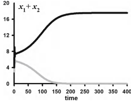
Figure 6.1: The total population sizes x_1(t) + x_2(t) of two solutions of the juvenile-adult model in Example 93 with density factors (6.29) with parameter values \mathcal{R}_0 = 0.85 , s_1 = 0.2 , s_{1m} = 0.4 , s_2 = 0.5 , c_1 = 0.05 , c_2 = 1 , which yield \kappa = -0.003 . The solution with initial condition (x_1(0), x_2(0))^T = (4, 0)^T (shown in black) approaches the positive equilibrium (10.773, 6.791)^T while that with initial condition (x_1(0), x_2(0))^T = (3, 0)^T (shown in gray) approaches the extinction equilibrium (0, 0)^T .
