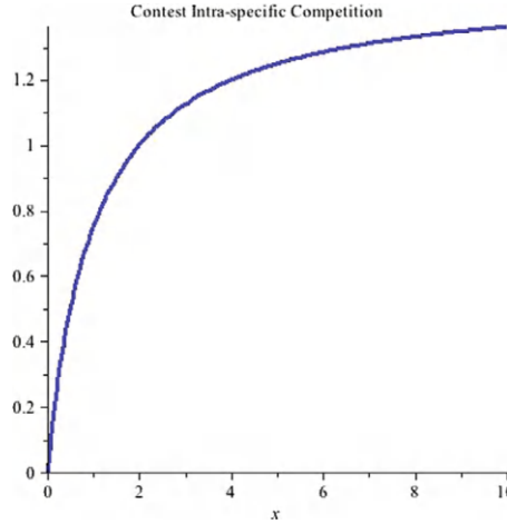
Figure 1.6: A contest competition model.
