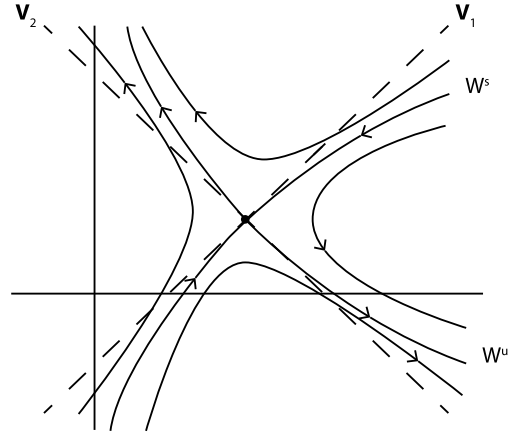
(b) The phase space diagram of the nonlinear system \mathbf{x}(t+1) = F(\mathbf{x}(t)) .
