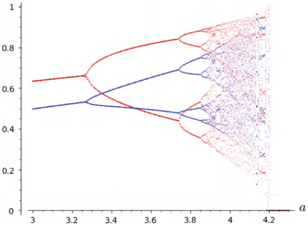
Figure 3.42: Period-doubling route to chaos is shown.
