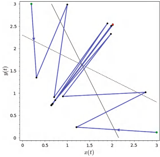
Figure 3.21: A phase space diagram showing a locally asymptotically 2-cycle.
