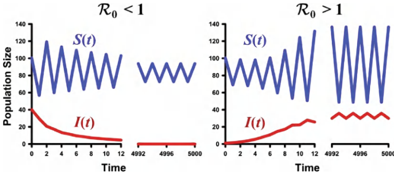
Figure 7.6: Sample solution times series from the SI model (7.53) with escape function (7.57) and parameter values b = 30 , c = 5/100 and c_S = 1/2 , c_I = 2/5 . Left plot: c_\varphi = 11/10 and \rho_2^* = 361/400 \approx 0.90 ( \mathcal{R}_0 = 11/12 \approx 0.92 ). Right plot: c_\varphi = 12/5 = 2.4 and \rho_2^* = 64/25 \approx 2.56 ( \mathcal{R}_0 = 2 ).
