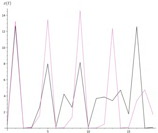
Figure 1.24: The error almost doubles after each iteration.
