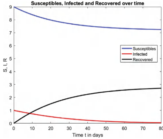
Figure 4.3: In model (4.2), the densities of susceptible and infected decrease monotonically while that of the recovered increases monotonically.
