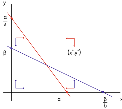
Figure 3.30: If a\beta < \alpha < \frac{\beta}{b} , the isoclines of system (3.79) intersect in the first quadrant guaranteeing the existence of a positive equilibrium (x^*, y^*)^T .
