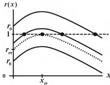
Figure 5.8: Plotting r(x) versus x illustrates the two cases: (I) r(0) < 1 , r(x_m) < 1 , r(x_m) = 1 , f(x_m) > 1 and (II) r(0) > 1 , r(0) = 1 .
