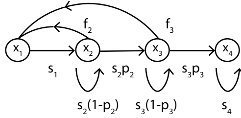
Figure 2.6: The life cycle graph of the Leslie matrix model in Example 24.
