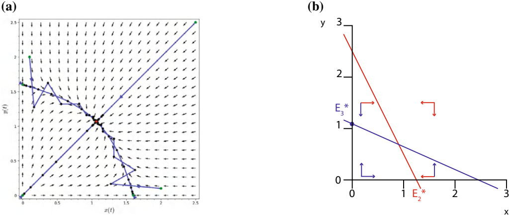
Figure 3.14: (a) The equilibrium points E_4^* is locally asymptotically stable and both E_2^* and E_3^* are saddle points. (b) The isoclines intersect at the coexistence equilibrium point E_4^* . The orientation of the orbits indicate that E_4^* is most likely asymptotically stable.
