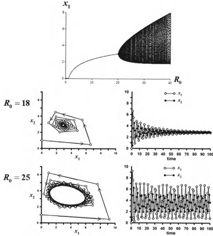
Figure 6.6: The bifurcation diagram for the k = 2 dimensional matrix model with the Leslie projection matrix (6.51) with f_3 = \mathcal{R}_0(1 - s_2)/s_1 and s_1 = s_2 = 0.5 and c = 1 show a Neimark-Sacker bifurcation to an invariant loop at \mathcal{R}_0^* = e^3 \approx 20.09 . A sample orbit with initial condition \mathbf{x}(0) = (0, 1)^T is displayed in the phase plane and in time series for a value of \mathcal{R}_0 = 18 before the bifurcation and \mathcal{R}_0 = 25 after the bifurcation.
