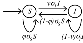
Figure 4.6: The compartmental diagram for the SI model (4.15).
