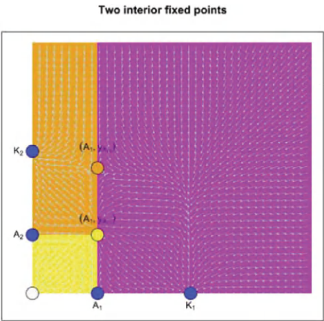
Figure 5.18: The phase space diagram in the case of two interior fixed points. The domain \mathbb{R}_+^N is divided into three regions, an extinction region (yellow), an exclusion region of y (magenta), and an exclusion region of x (orange). Note that the extinction region is bounded.
