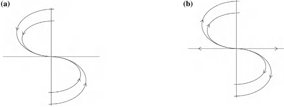
Figure 3.2: (a) a degenerate sink: \lambda_1 = \lambda_2 = \lambda, \lambda < 1 . (b) a degenerate source: \lambda_1 = \lambda_2 = \lambda, \lambda > 1 .
