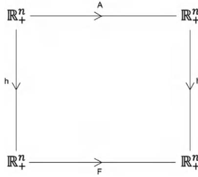
Figure 3.23: The map F is conjugate to A = JF(\mathbf{x}^*) , that is, F(h(\mathbf{x})) = h(A\mathbf{x}) .
