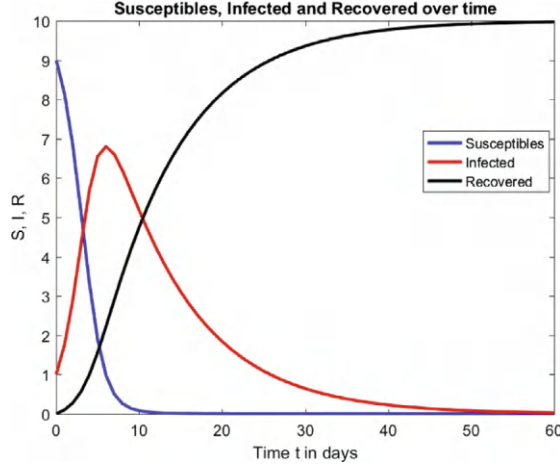
Figure 4.2: In model (4.2), the density of susceptibles decreases monotonically, density of recovered increases monotonically, while that of infected initially increases to a maximum value before decreasing to zero.
