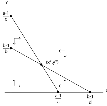
Figure 3.40: Isoclines: The coexistence equilibrium E_4^* exists if \frac{a-1}{c} > \frac{b-1}{b} and \frac{b-1}{d} > \frac{a-1}{a} , a > 1 , b > 1 .
