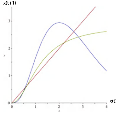
Figure 5.7: The green curve represents a contest competition model with the strong Allee effect while the blue curve represents a scramble competition model with the strong Allee effect.
