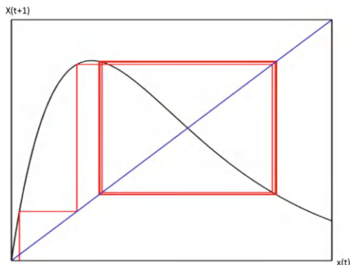
Figure 1.12: The cobweb diagram of the Ricker map where \alpha = 2.2 . The positive equilibrium point x_2^* = \alpha is unstable. The population fluctuates around two values.
