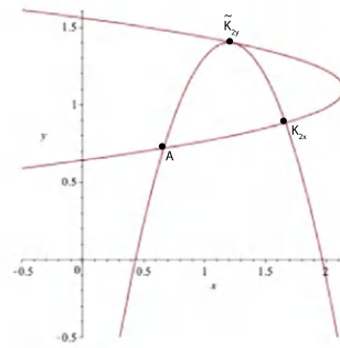
(e) a_1 = 2.4 , a_2 = 2.2 , b_1 = 0.4208 , b_2 = 0.0978 Three interior equilibria.
