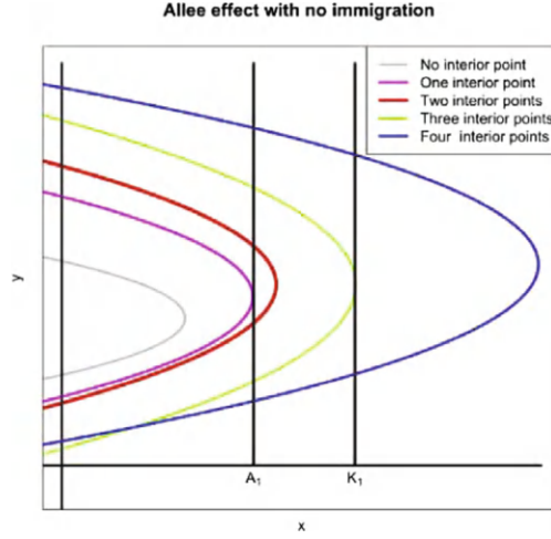
Figure 5.16: The five scenarios of the Allee effect. The graph depicts the various curves of the second isocline (parabola). The interior fixed points are the intersection of the second isocline with the isoclines x = A_1 and x = K_1 . The five scenarios are (i) no interior fixed points, (ii) one interior fixed point, (iii) two interior fixed points, (iv) three interior fixed points, (v) four interior fixed points.
