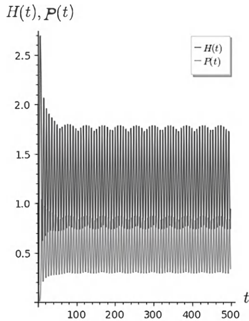
Figure 3.38: Time-series plots of H(t) and P(t) versus t , for the parameters r = 1.25 , \alpha = 1 , c = 1 , and K = 2.7 .
