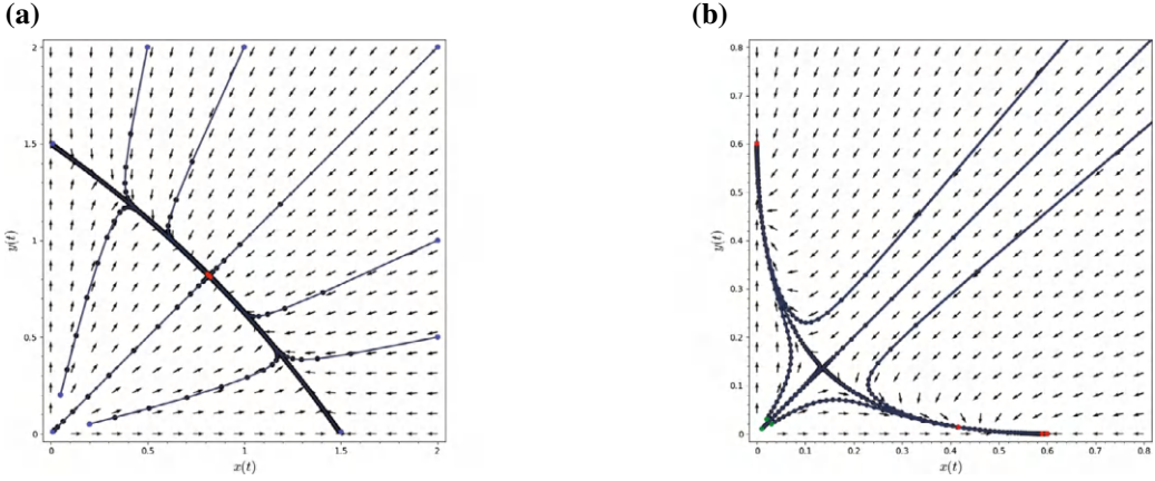
Figure 3.12: (a) The phase space diagram of the Leslie–Gower model: E_1^* is a repeller (unstable), E_2^* and E_3^* are saddle points, while E_4^* is asymptotically stable. (b) The phase space diagram of the Leslie–Gower model: E_4^* is a saddle, E_2^* and E_3^* are locally asymptotically stable.
