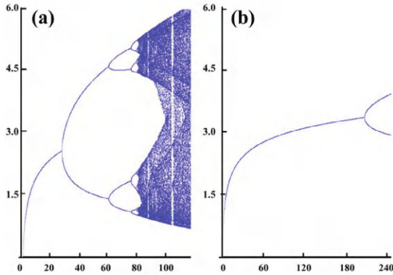
Figure 8.11: The bifurcation diagram showing the x component of the Darwinian Ricker equation with c_0 = 1 , and (a) c_1 = 0.5 and \sigma^2 = 0.5 and (b) c_1 = 0.6 and \sigma^2 = 0.5 .
