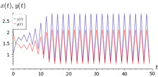
Figure 3.20: Time series showing a 2-cycle.
