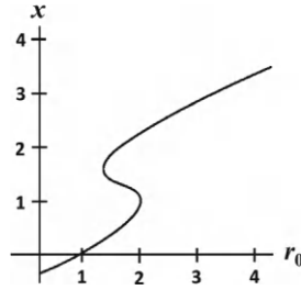
Figure 1.15: The bifurcation diagram associated with Equation (1.47) with parameter values v = 4 , u = 1.5 , c = 2 , and m = 4 shows a forward bifurcation at r_0 = 1 and a hysteresis shape with multiple positive equilibria for r_0 between approximately 1.4 and 2.0.
