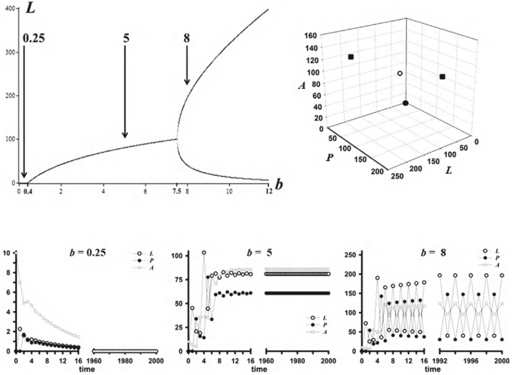
Figure 6.7: Shown is the bifurcation diagram for the LPA model with projection matrix (6.53), using b as the bifurcation parameter, and plotting the L component of the attractor. Parameter values are c_{el} = c_{eq} = c_{pa} = 0.01 , \mu_l = 0.25 , and \mu_a = 0.3 . The forward, stable bifurcation of positive equilibria occurs at b_0 = 0.4 and a 2-cycle bifurcation occurs at b \approx 7.5 . The upper right plot shows three sample attractors in phase space: the extinction equilibrium (solid dot) when b = 0.25 ; a positive equilibrium (open dot) when b = 5 ; and 2-cycle (open squares) when b = 8 . Sample solution time series (with initial condition \mathbf{x}(0) = (L, P, A)^T = (0, 0, 10) ) are shown for each of these three cases in the bottom row.
