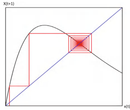
Figure 1.11: The cobweb diagram of the Ricker map where \alpha = 1.9 . The population approaches the positive equilibrium point x_2^* = \alpha . The extinction equilibrium x_1^* = 0 is unstable, while x_2^* is attracting.
