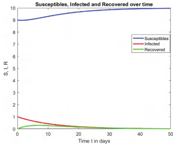
Figure 4.5: In model (4.10), \mathcal{R}_0 = 0.2 , and the disease-free equilibrium point, (S^*, I^*, R^*)^T = (10, 0, 0)^T is asymptotically stable.
