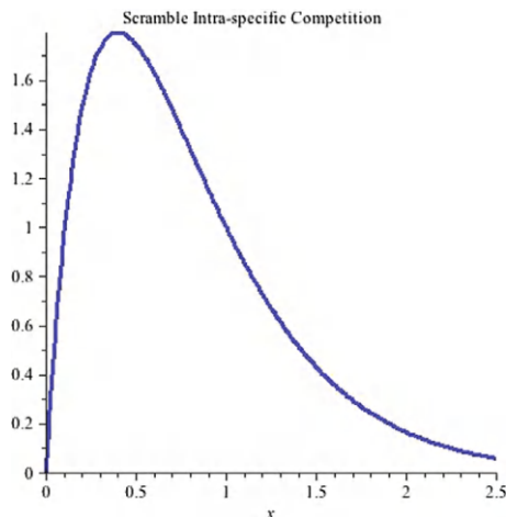
Figure 1.7: A scramble competition model.
