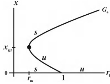
Figure 5.9: The backward bifurcation near the bifurcation point (r_0, x) = 1 .
