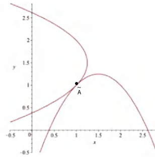
(b) a_1 = 3 , a_2 = 3 , b_1 = 1 , b_2 = 1 One interior equilibrium point.
