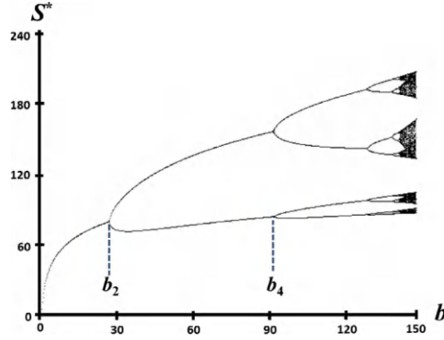
Figure 7.5: Period-doubling bifurcations in model (7.53) with escape function (7.57) and parameter values c = 0.05 and \sigma_S = 0.5 . For 0.5 < b < b_2 there is a stable equilibrium and for b_2 < b < b_4 there is a stable 2-cycle where b_2 \approx 27.3 and b_4 \approx 92.2 .
