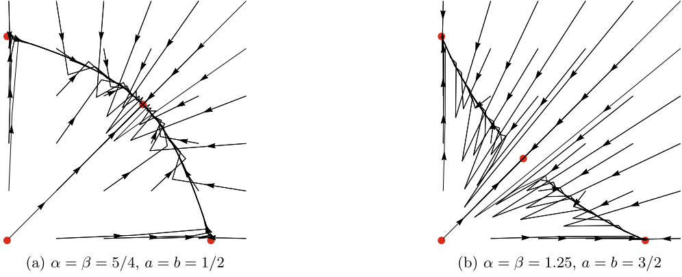
Figure 3.25: Examples of dynamics catalogued in Theorem 30.
