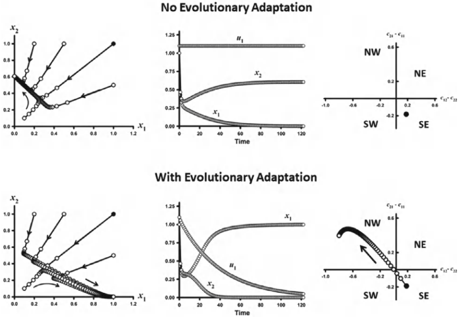
Figure 8.8: Shown are the results of simulations of the Darwinian Leslie–Gower model (8.32) with coefficients (8.33) and (8.34) and with parameter values b = 2 , a = 1 , u_2 = 1 , \sigma_k^2 = 1 , and \sigma_\alpha^2 = 3 . Top row: In these plots, \sigma_1^2 = 0 and there is no adaptive evolution. The graph of the left shows the (x_1(t), x_2(t))^T components, in the (x_1, x_2) -plane, from five solutions (x_1(t), x_2(t), u_1(t))^T with the initial conditions (x_1(0), x_2(0), u_1(0))^T = (1, 1, 1.1)^T , (0.2, 1, 1.1)^T , (0.5, 1, 1.1)^T , (1, 0.5, 1.1)^T , and (0.1, 0.1, 1.1)^T . Note that species x_1(t) goes extinct and \lim_{t \rightarrow \infty} x_2(t) = 0.6065 . The time series for the solution with the first initial condition (shown by the black dot) is shown in the middle graph. The right-hand graph shows that the point P(1, 1, 1.1) lies in the SE quadrant. Bottom row: In these plots, evolutionary adaptation of species x_1 occurs with \sigma_1^2 = 0.05 . Now species x_2(t) goes extinct while \lim_{t \rightarrow \infty} x_1(t) = 1 and the mean trait of x_1(t) evolves to 0. In this case, the point P(x_1(t), x_2(t), u_1(t)) migrates from the SE quadrant to the NW quadrant, demonstrating the reversal of the competitive outcome.
