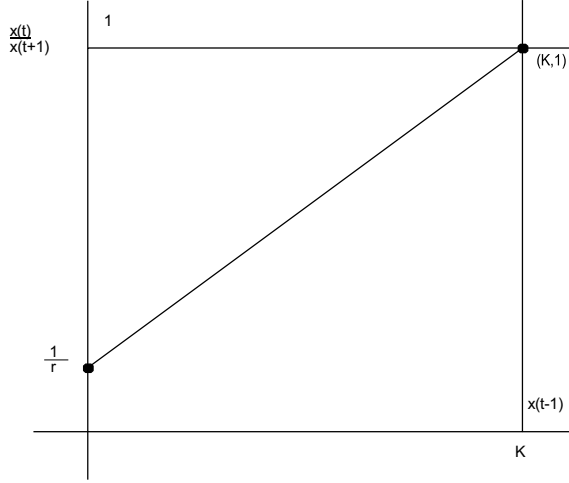
Figure 3.24: The graph depicts the reciprocal of the growth rate of the population r versus x(t-1) on the x -axis.
