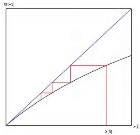
Figure 1.8: The cobweb diagram of the discrete logistic map where b \leq 1 . The population goes extinct.
