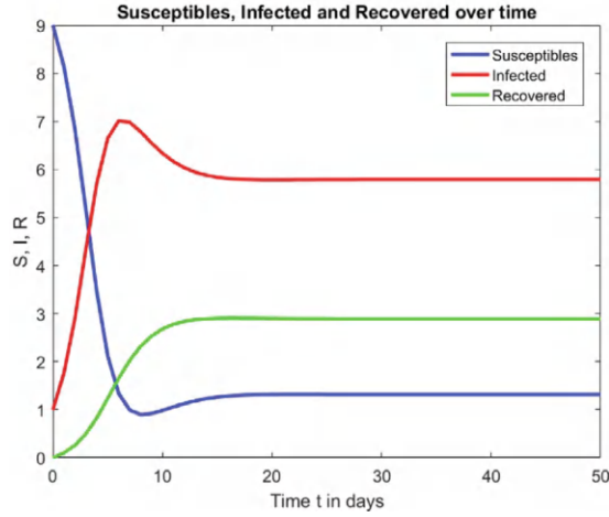
Figure 4.4: In model (4.10), \mathcal{R}_0 = 10 , and there is an asymptotically stable endemic equilibrium point at (S^*, I^*, R^*)^T = (1.3172, 5.7885, 2.9843)^T .
