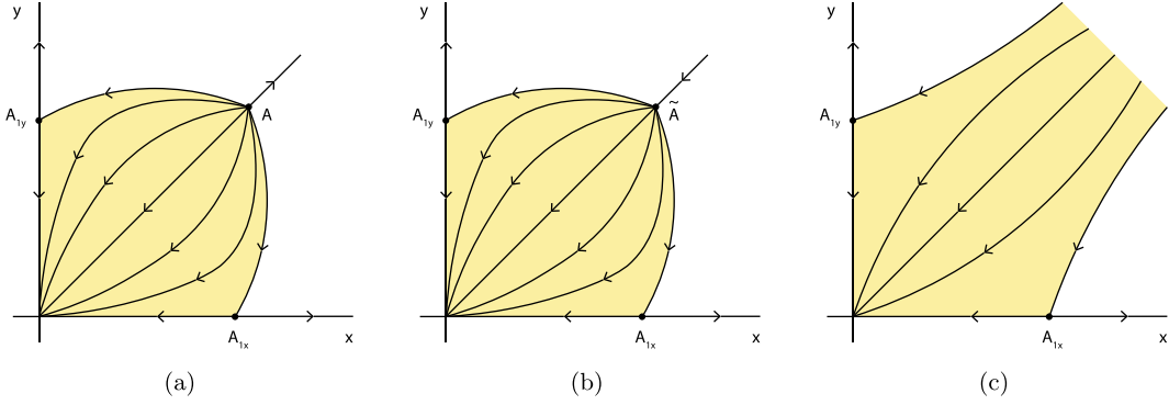
Figure 5.11: There are two possible rearrangements of the equilibrium along the Allee threshold curve (a,b) and one possibility of no interior equilibrium points, where the extinction region is unbounded (c).
