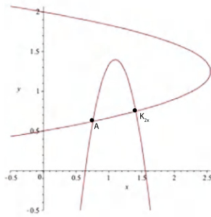
(d) a_1 = 2.2 , a_2 = 2.5 , b_1 = 0.15 , b_2 = 0.22 Two interior equilibria.
