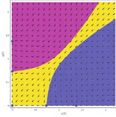
(a) no interior equilibrium points
