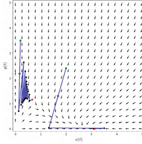
Figure 5.1: The graph shows two attractors, an equilibrium point on the x -axis, and a 2-cycle in the interior.
