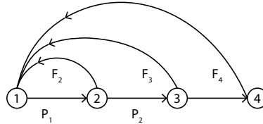
Figure 3.6: The chart depicts four age classes n_1 , n_2 , n_3 and n_4 , where P_i is the probability an individual in age class i , 1 \leq i \leq 3 , is alive at time t+1 , and F_i is the fertility rate of n_i .
