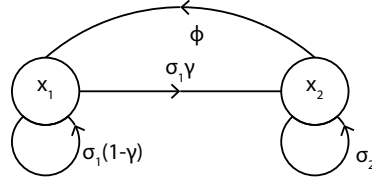
Figure 3.29: The life cycle graph of model (3.74).
