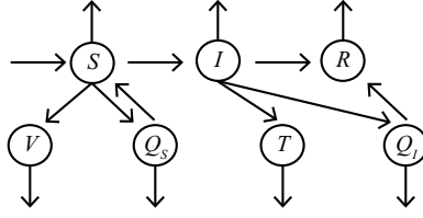
Figure 4.7: SIR Model with Vaccination and Quarantine.
