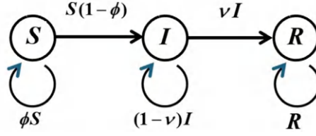
Figure 4.1: Flowchart for Discrete-time Kermack-McKendrick SIR model.
