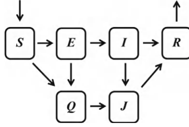
Figure 7.9: Flowchart for Discrete-Time SARS model.
