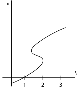
Figure 5.10: A forward bifurcation at r_0 = 1 with a hysteresis loop that creates the existence of multiple positive equilibria for an interval of r_0 values.
