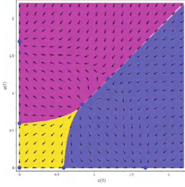
(c) two interior equilibrium points
