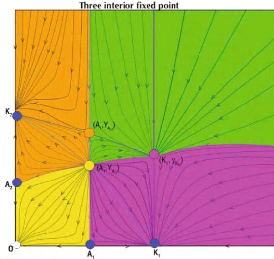
Figure 5.21: The phase space diagram in the case of three interior fixed points. The domain \mathbb{R}_+^2 is divided into four regions: an extinction region (yellow), an exclusion region of y (magenta), an exclusion region of x (orange), and a coexistence region (green). Note that this is the first instance when we have a coexistence region.
