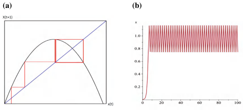
Figure 1.19: (a) Cobweb. Asymptotically stable 2-cycle, r = 2.2 . (b) Time series. Asymptotically stable 2-cycle in (t, x_t) -plane, r = 2.2 .
