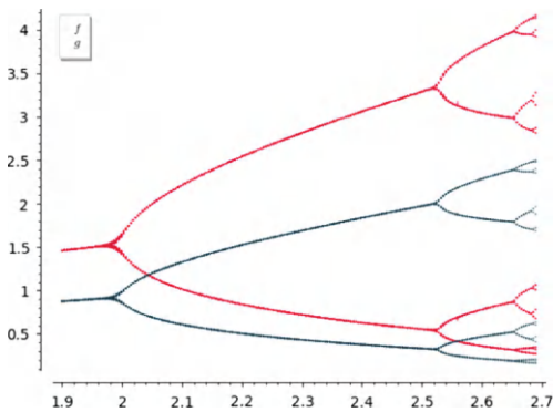
Figure 3.33: The Ricker map F is written as F = (f, g) . The figure shows a bifurcation diagram, on the x-axis we have the parameter \alpha and on the y-axis we have the omega limit sets of both the x-components and the y-components of the orbits.
