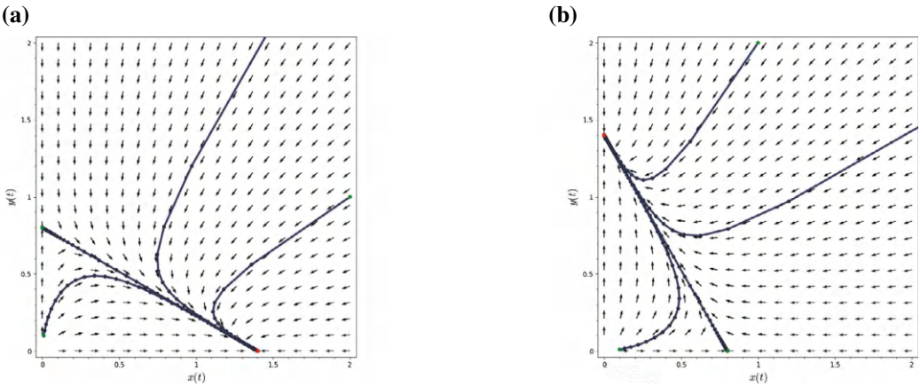
Figure 3.13: (a) The phase space diagram of the Leslie–Gower model: The equilibrium points E_2^* is locally asymptotically stable and E_3^* is a saddle. (b) The phase space diagram of the Leslie–Gower model: The equilibrium points E_3^* is locally asymptotically stable and E_2^* is a saddle.
