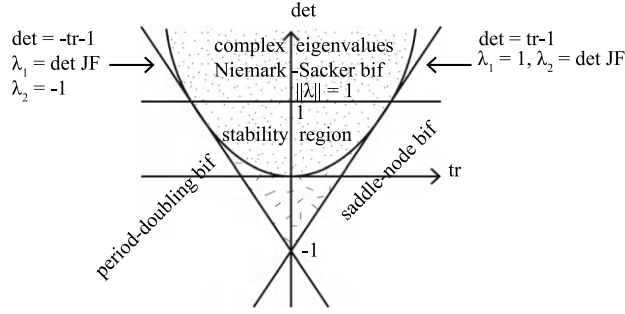
Figure 3.31: The det-tr figure showing the three main types of bifurcations on a two-dimensional map.
