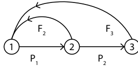
Figure 3.5: The chart depicts three age classes n_1 , n_2 and n_3 , where P_i is the probability an individual in age class i , 1 \leq i \leq 2 , is alive at time t+1 , and F_i is the fertility rate of n_i .
