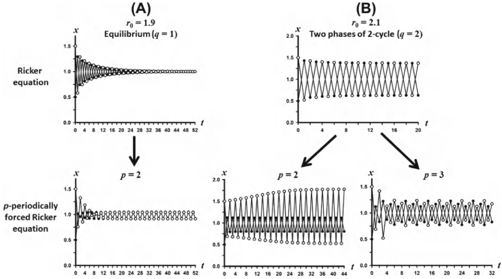
Figure 9.1: In each plot there is shown two times-series solutions, with initial conditions x(0) = 0.5 and 1.5 , of the Ricker p -periodically forced Ricker (9.32) with coefficients (9.38) and K_0 = 1 and \alpha_r = -50 . The two row plots are without periodic forcing, i.e., \alpha = 0 and the bottom row are plots with small amplitude forcing \alpha = 0.01 . (A) With r_0 = 1.9 the unperturbed Ricker equation has a hyperbolic, stable equilibrium (i.e., a q = 1 periodic solution) which, when p = 2 periodically forced, results in a stable 2-periodic solution. (B) With r_0 = 2.1 the unperturbed Ricker equation has a hyperbolic, stable q = 2 periodic solution which has two phase shifts. The upper plot shows one of the computed solutions ( x(0) = 0.5 ) tending to one phase of the 2-cycle and the other ( x(0) = 1.5 ) tending to the other phase of the 2-cycle. When forced with period p = 2 (lower left plot) we see the two initial conditions tending to two 2-periodic solutions which are not phase shifts of each other. When forced with period p = 3 (lower right plot) we see the two initial conditions tending to two 6-periodic solutions ( m = 6 is the least common multiple of 2 and 3) which are not phase shifts of each other.
