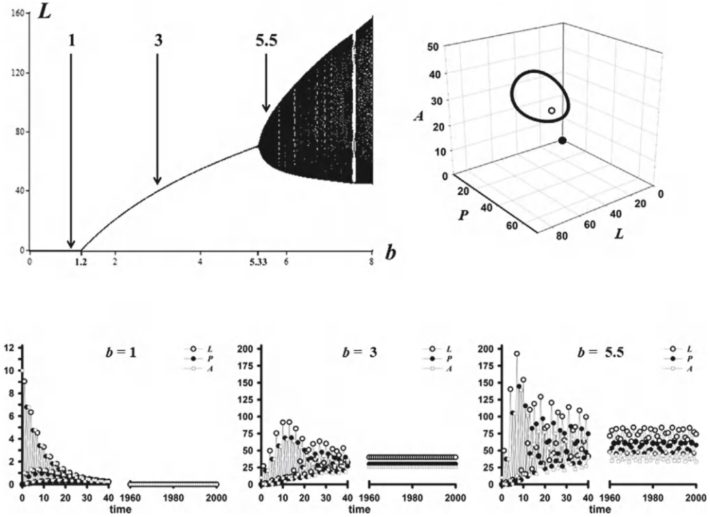
Figure 6.8: Shown is the bifurcation diagram for the LPA model with projection matrix (6.53), using b as the bifurcation parameter, and plotting the L component of the attractor. Parameter values are c_{el} = c_{eq} = c_{pa} = 0.01 , \mu_l = 0.25 , and \mu_a = 0.9 . The forward, stable bifurcation of positive equilibria occurs at b_0 = 1.2 and a Neimark-Sacker bifurcation to an invariant loop occurs at b \approx 5.33 . The upper right plot shows three sample attractors in phase space: the extinction equilibrium (solid dot) when b = 1 ; a positive equilibrium (open dot) when b = 3 ; and an invariant loop when b = 5.5 . Sample solution time series (with initial condition \mathbf{x}(0) = (L, P, A)^T = (0, 0, 10) ) are shown for each of these three cases in the bottom row.
