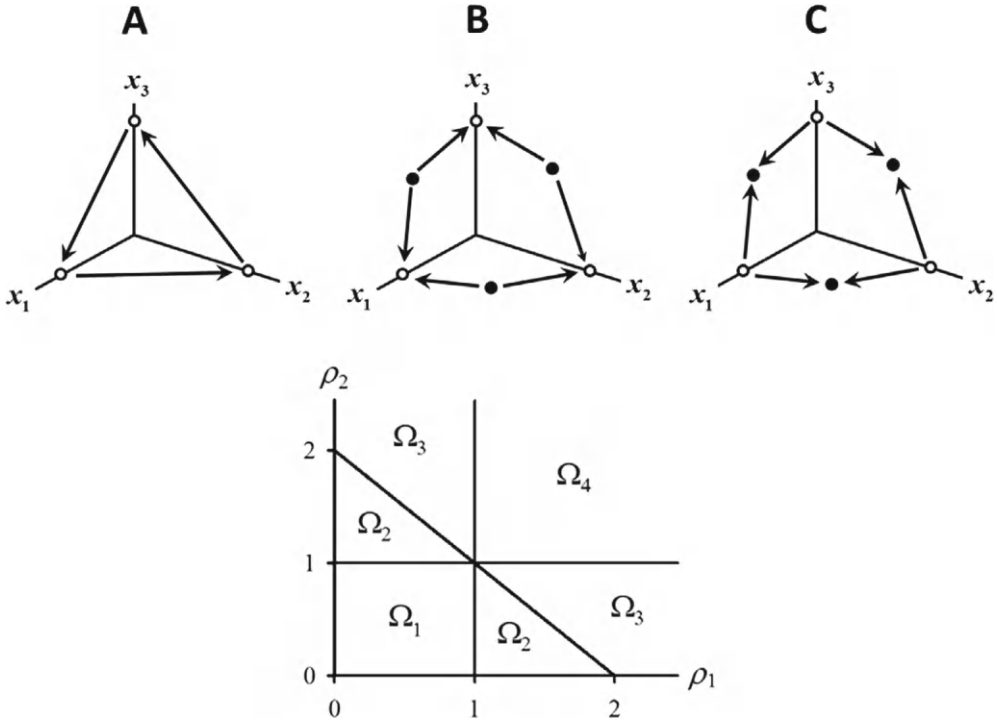
Figure 6.4: For \mathcal{R}_0 \gtrsim 1 in the k = 3 dimensional semelparous Leslie model with projection matrix (6.49), there exist an invariant loop of one of the three geometries shown. In the \rho_1 and \rho_2 parameter region \Omega_2 \cup \Omega_3 , the loop is of type A. In region \Omega_4 , the loop is of type B and in region \Omega_1 it is of type C. The open regions \Omega_i in the (\rho_1, \rho_2) -plane are defined in the lower graph. The open circles on the coordinate axes are the fixed points of the composite map and correspond to the three different phases of a single-class 3-cycle. In types B and C, the solid circles interior to the coordinate planes are also fixed points of the composite map, but correspond to the three phases of a two-class 3-cycle. The oriented connecting lines are heteroclinic orbits that connect the phase shifts of these 3-cycles. The temporal motion is counter-clockwise, visiting the coordinate planes sequentially. Figure reproduced with permission from [71].
