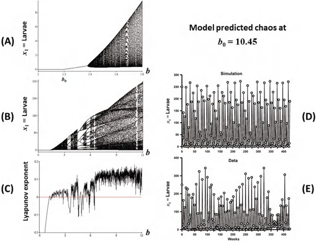
Figure 6.11: The same plots are shown as in Figure 6.10 but with c_{pa} changed from 0.5 to 0.35. At b = 10.45 the predicted attractor is now chaotic.
