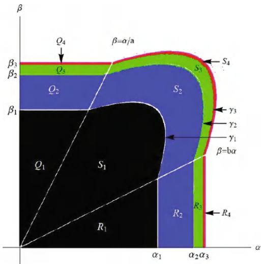
Figure 3.32: A parameter space (\alpha, \beta) bifurcation diagram for system (3.81) which shows period-doubling in the three regions Q_1 (where species x goes to extinction), S_1 (where the coexistence equilibrium is asymptotically stable), and R_1 (where species y goes to extinction).
