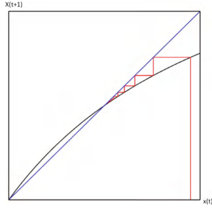
Figure 1.10: The cobweb diagram of the discrete logistic map, where b > 1 . The population size approaches the equilibrium point.
