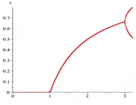
Figure 1.17: The bifurcation diagram of the quadratic map, at r = 1 we have a transcritical bifurcation, and at r = 3 , we have period-doubling bifurcation.
