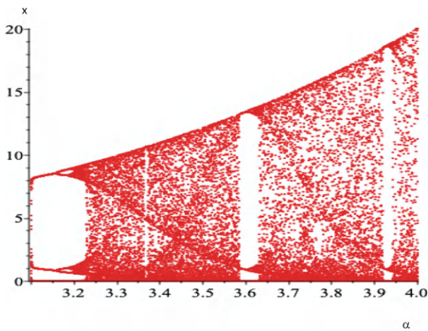
Figure 1.23: The appearance of odd periods and the “maximum” chaos at \alpha = 4 .
