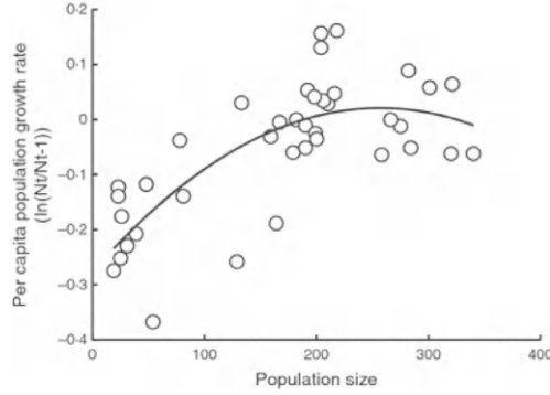
Figure 5.5: Annual counts of free-living V. I. marmots reveal strong inverse density dependence in per capita population growth from 1970 to 2007.
