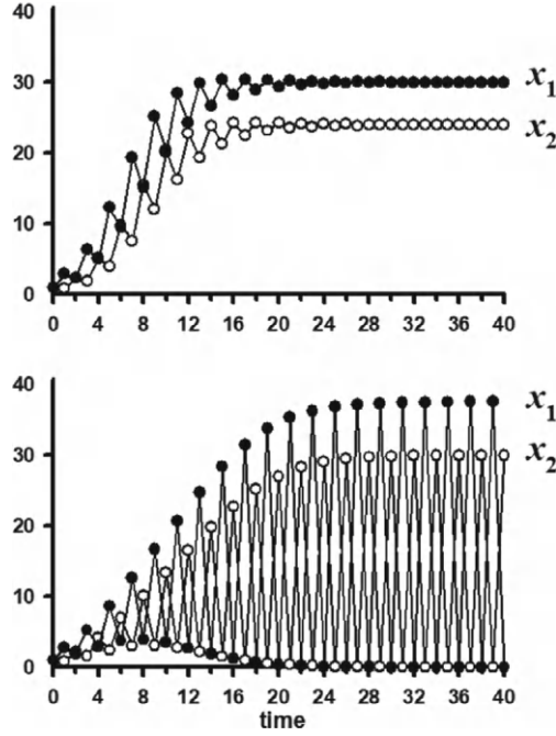
Figure 6.2: A sample solution, with initial condition (x_1(0), x_2(0))^T = (1, 1)^T of the model equation in Examples 94 and 95 with coefficients \mathcal{R}_0 = 2.5 , s = 0.5 and c_{22} = 0.01 , is shown. In the upper plot, c_{21} = 0.01 so that c_{21}/c_{22} = 0.1 < s and the positive equilibrium is stable (and the synchronous 2-cycle is unstable). In the lower plot, c_{21} = 0.1 so that c_{21}/c_{22} = 1 > s and the 2-cycle is stable (and the positive equilibrium is unstable).
