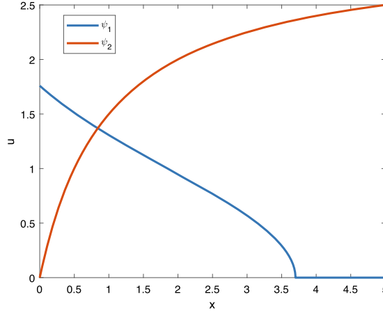
Figure 8.9: Existence of a unique positive fixed point for b_0 = 4.7 and c_1 = 3 .
