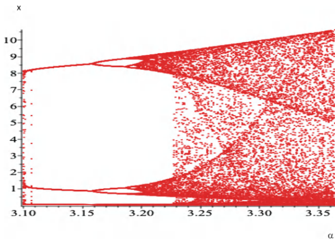
Figure 1.22: The appearance of period 3.
