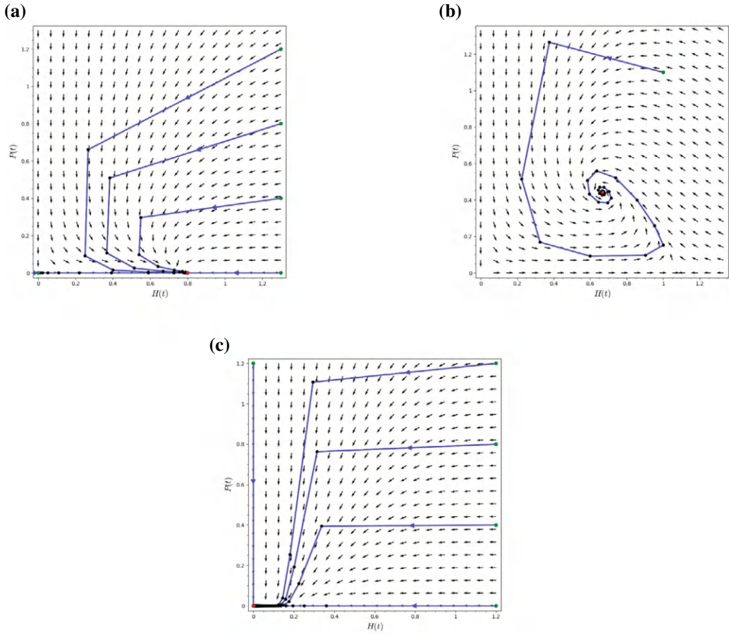
Figure 3.19: (a) 0 < r < 2, caK < 1 , E_2^* is asymptotically stable. (b) 0 < r < 2, caK > 1 , E_2^* is a saddle and E_3^* is asymptotically stable. (c) E_1^* = (0, 0) is asymptotically stable.
