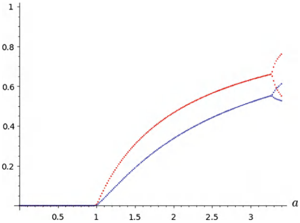
Figure 3.41: Shown is the bifurcation diagram for the symmetric version of the competition model (3.83). For 0 < a = b \leq 1 , the extinction equilibrium is asymptotically stable, and when a and b exceeds 1, a new asymptotically stable equilibrium point E_4^* is born.
