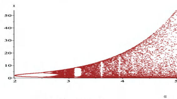
Figure (b): Bifurcation Diagram
